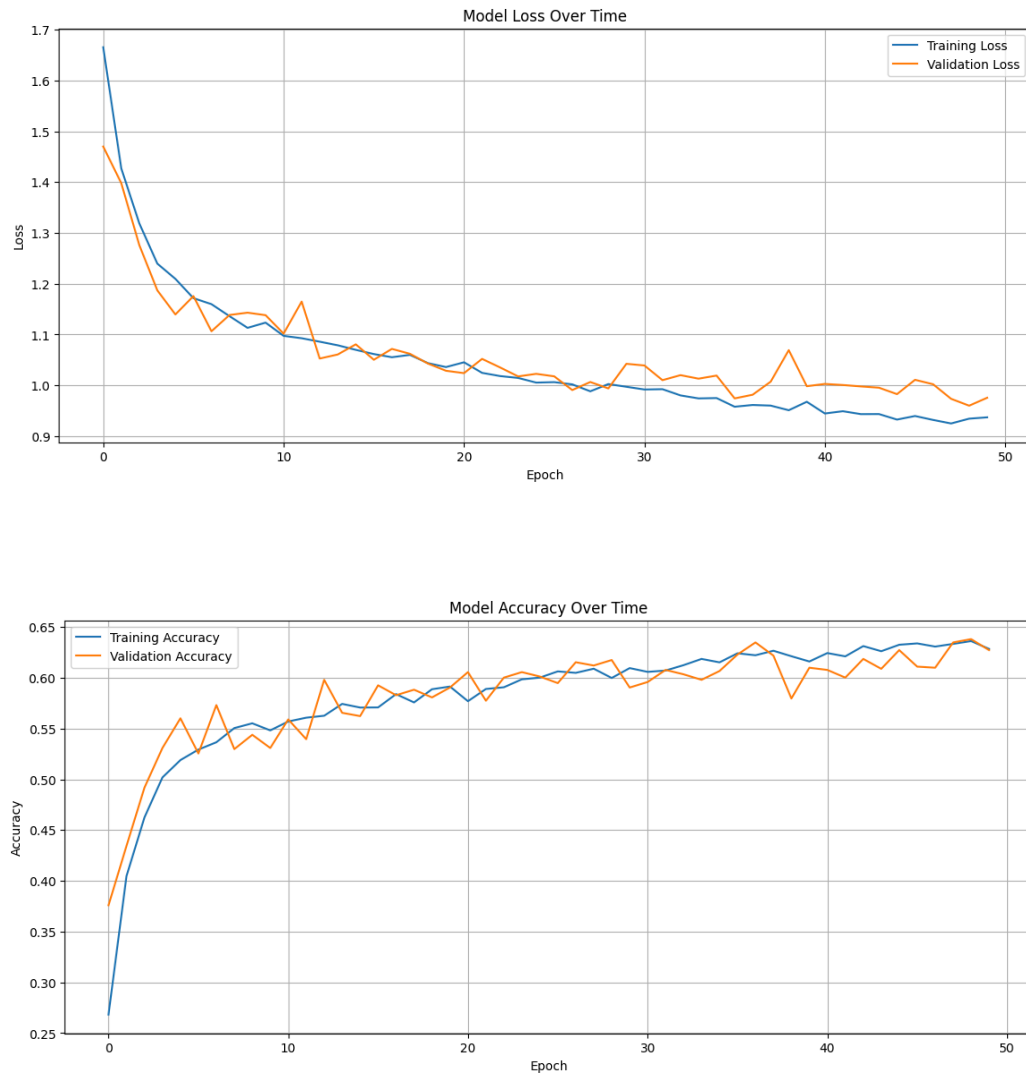
Figure 4.1.1.2 loss and accuracy curve Of RNN
