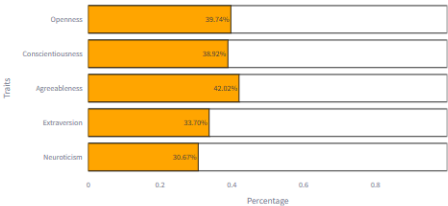
Personality Traits Percentage
