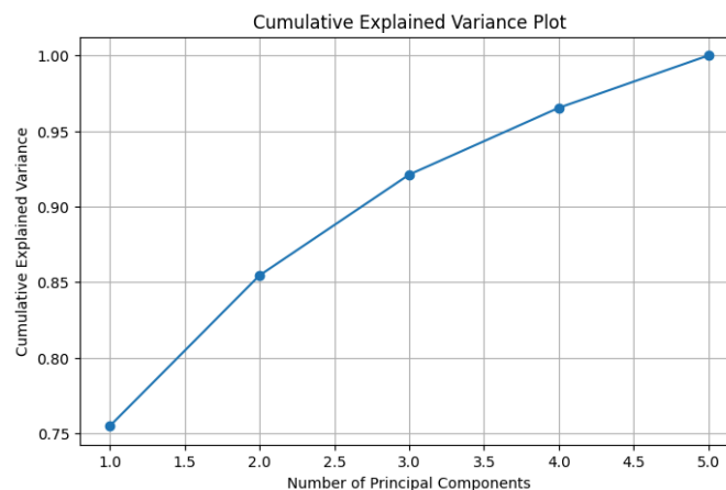
Figure 4.4.2 Cumulative Explained Variance Plot
